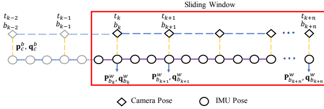
Fig. 3. Illustration of the sliding window used in the proposed system.
