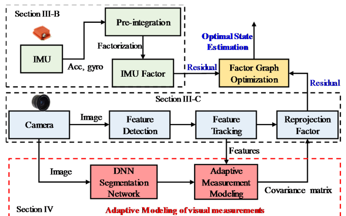
Fig. 2. Framework of the proposed VINS aided by adaptive modeling of visual measurements.
