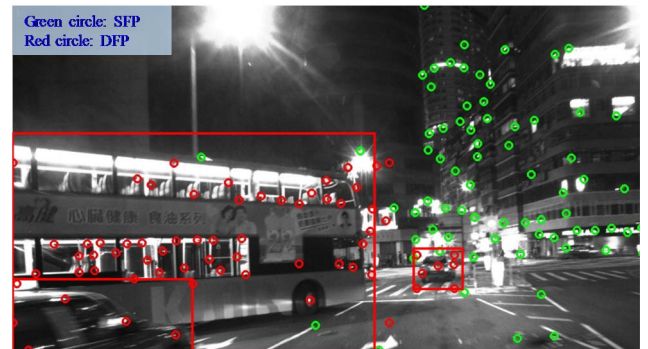
Fig. 6. Example of a case (Epoch 163) with numerous dynamic objects making up the majority of the image.
